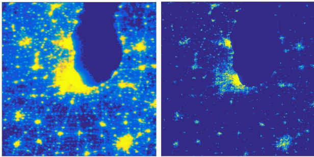
(a) DMSP-OLS
